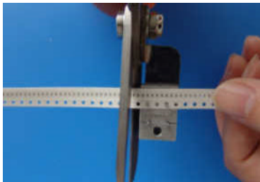
STEP 2: Place 4mm pitch tape on back set of locator pins for cutting.
