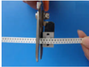
STEP 1: Place 8mm pitch tape on front set of locator pins for cutting.
